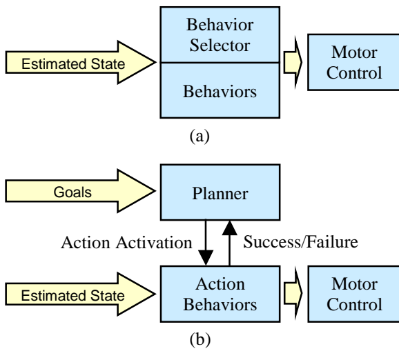
Figure 2. Comparing a universal plan (a) with a hybrid system (b)
