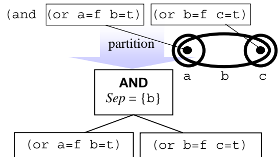
Figure 4. Example of partitioning a CNF equation
