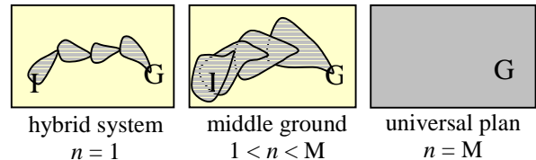
Figure 1. Parameterized state-space coverage – from a hybrid system to a universal plan
