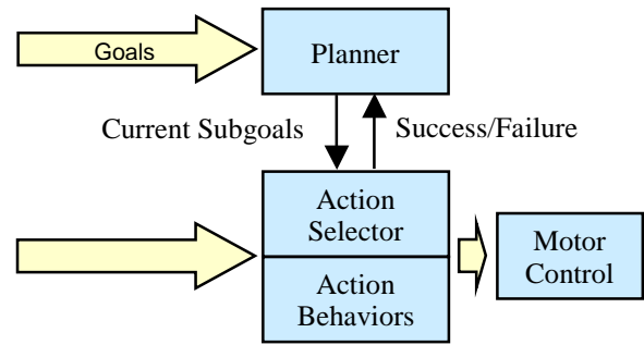
Figure 3. A universal( n ) system
